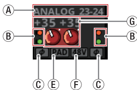
Input area display when the input source is "ANALOG" or "SB-16D connected by built-in Dante"
