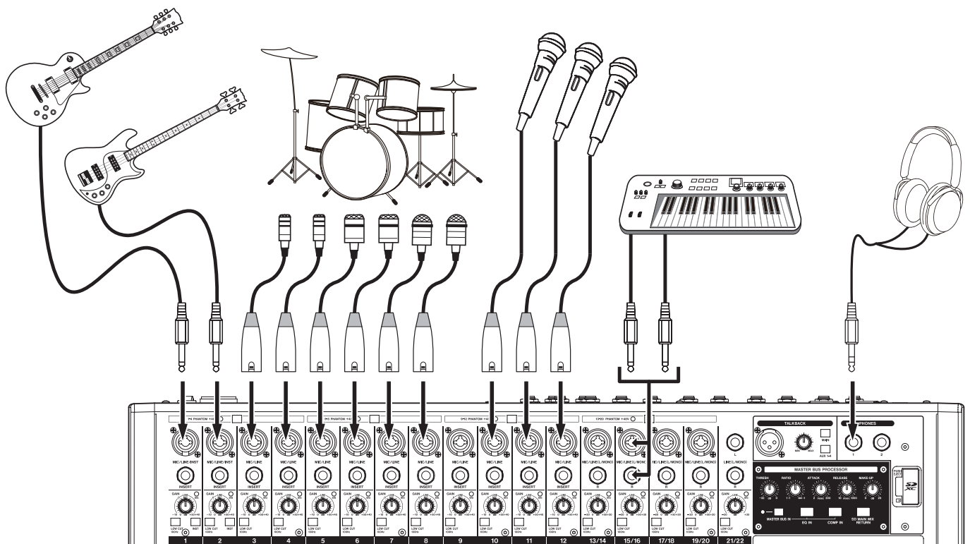
Examples of connections to a Model 2400
